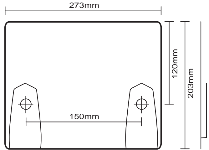
Code: 4906 Wall Mounted Steel Dispenser
