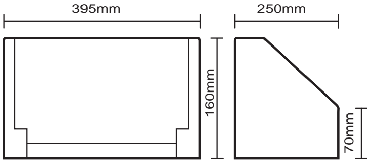
Code: 4920 Wall Mounted Dispenser
